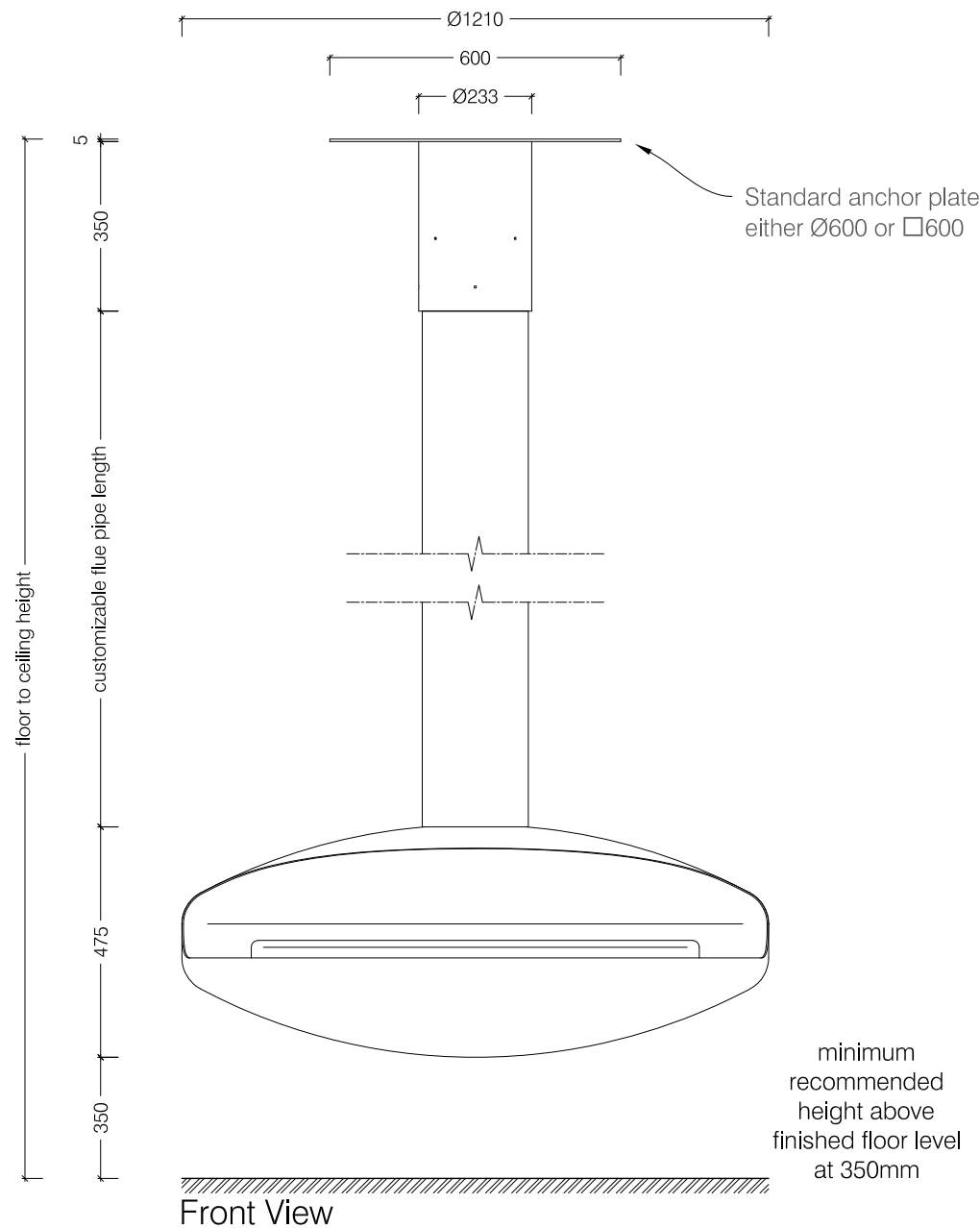
Float Ø1210 with Grand XL Burner
