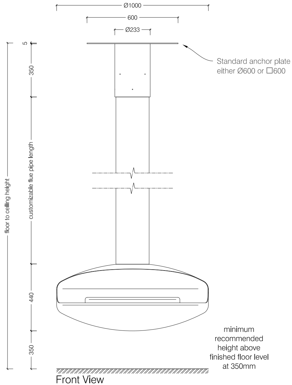
Float Ø1000 with Classic Burner
