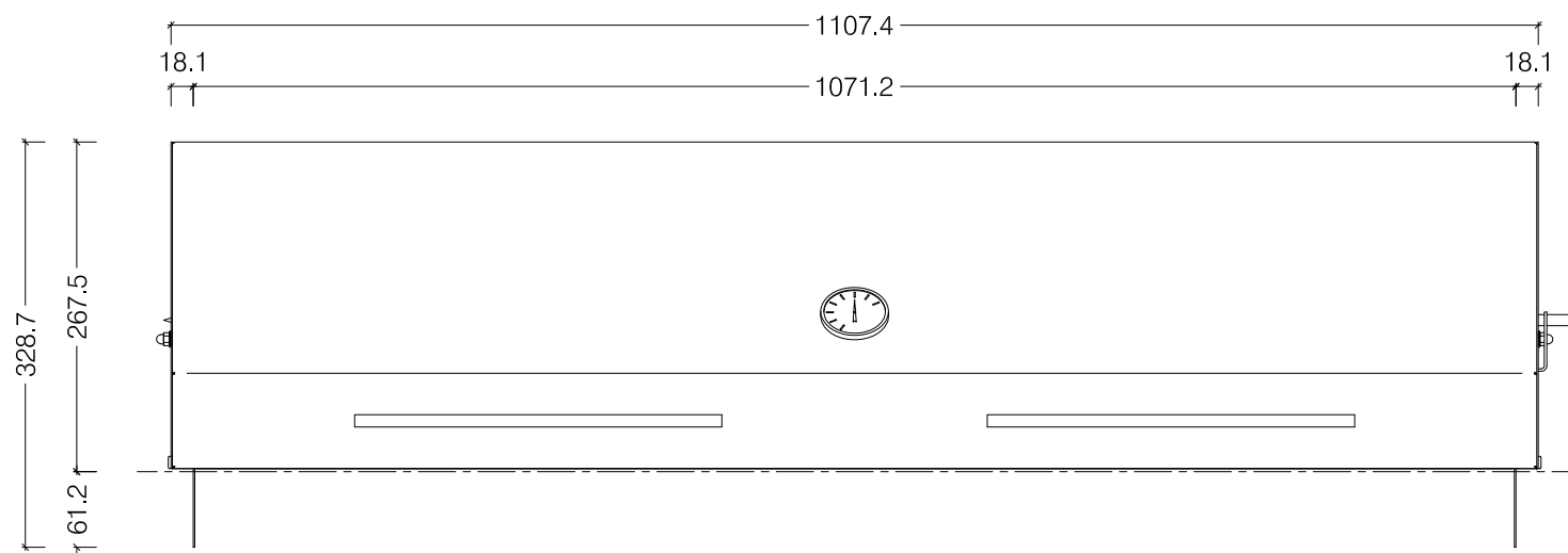
Front View
