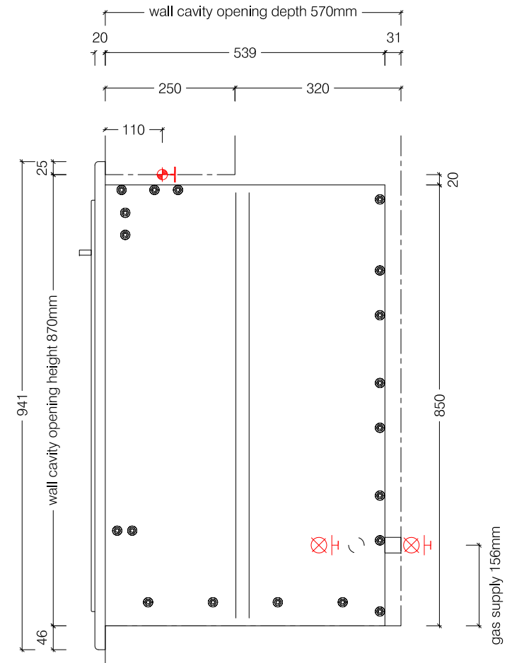
Side View
