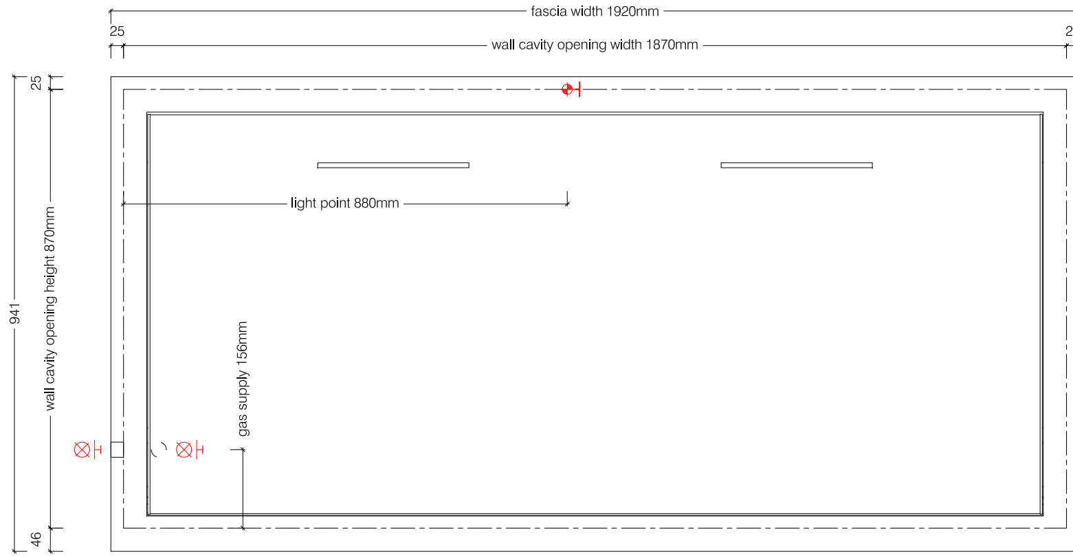
Front View
