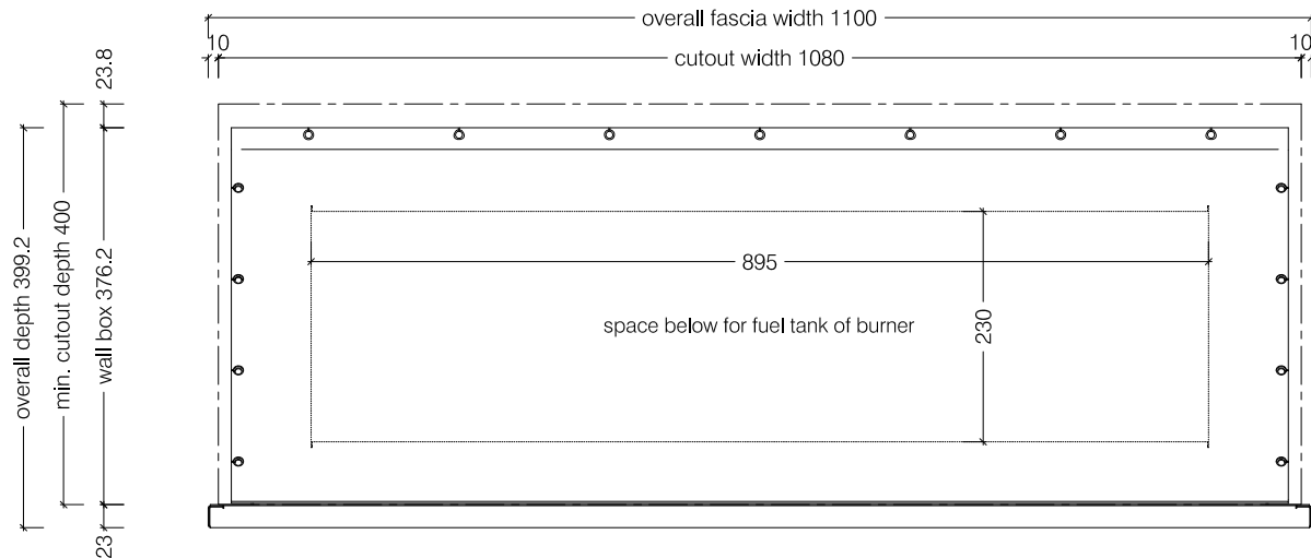
Top View
