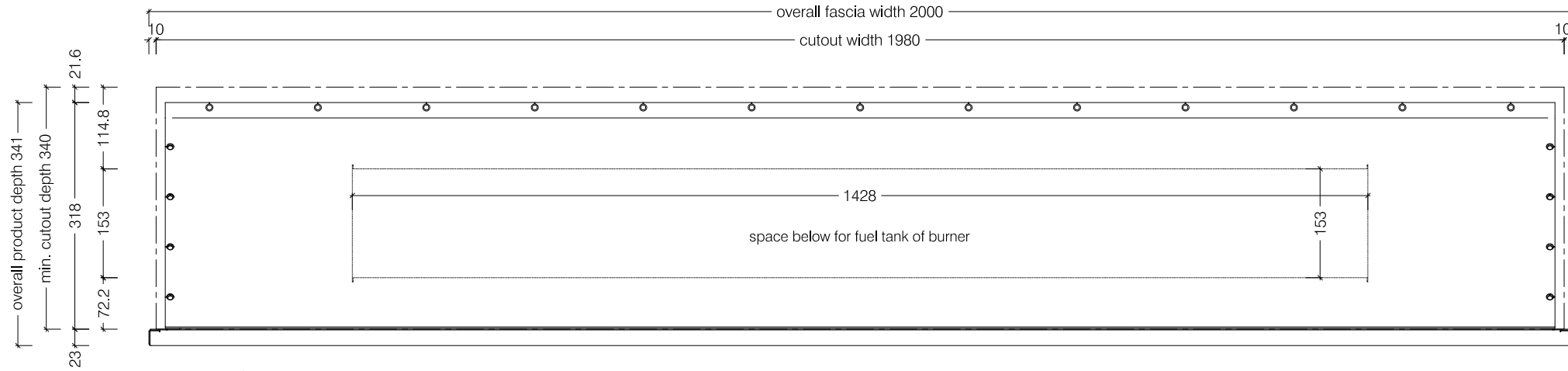
Top View
