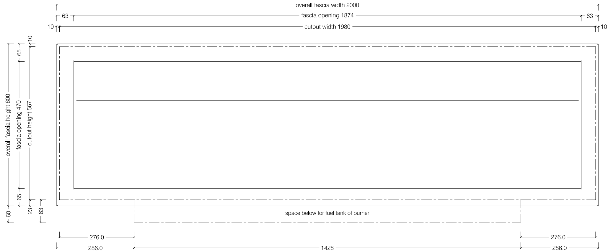
Front View
