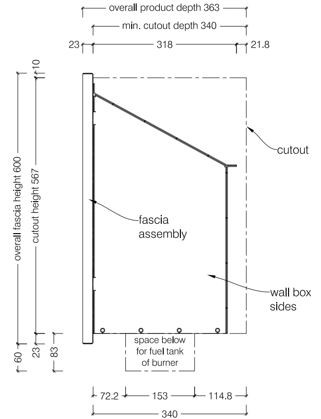
Side View
