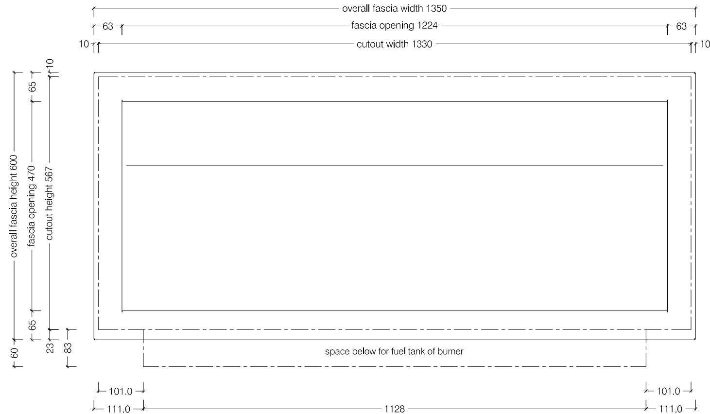
Front View
