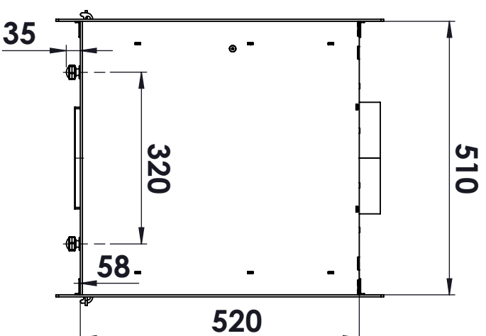
NICKEL 800 DS Opening Size Required 820mm L x 510mm D x 605mm H
